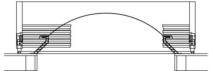
Frame with Topspin awnings 50 cm larger than light dome
